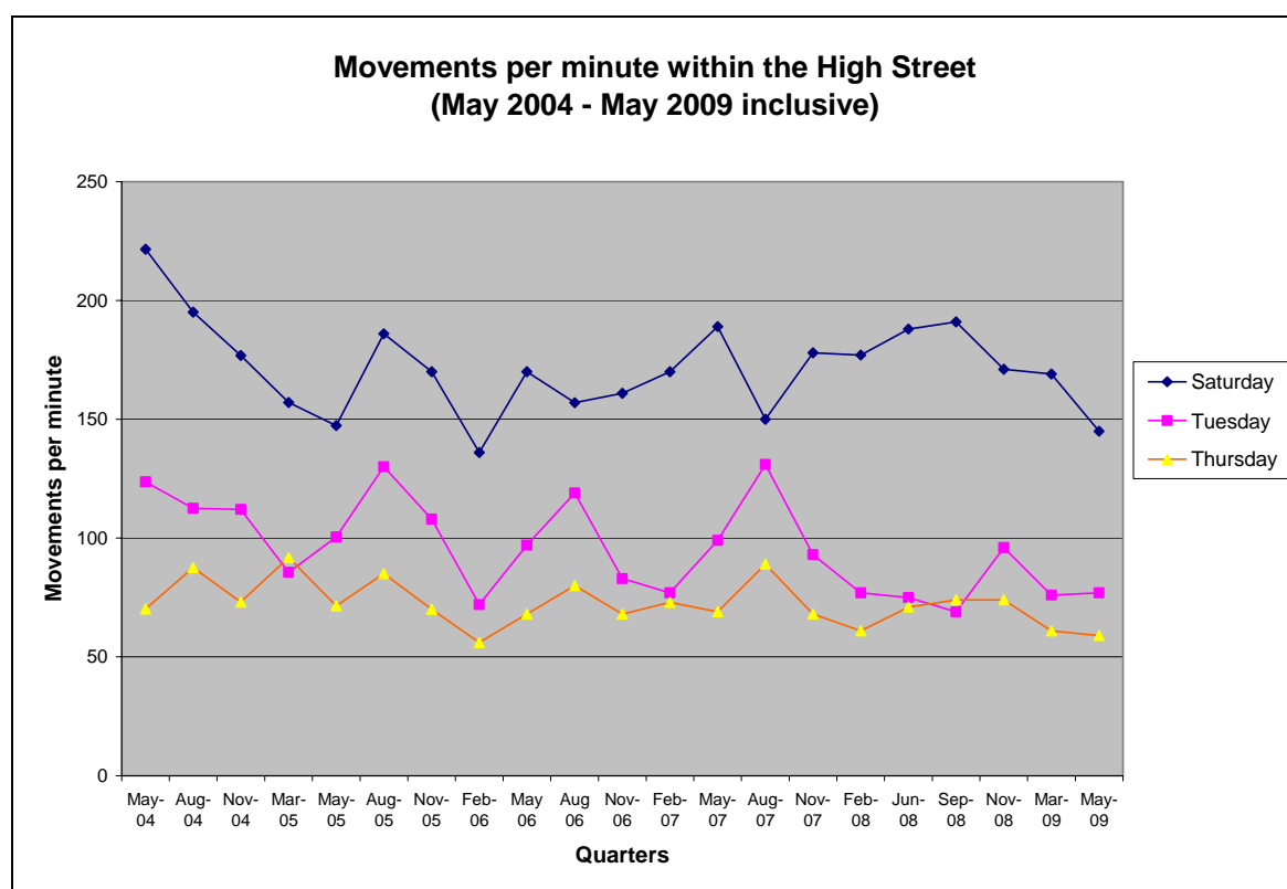
Figure 8.8: Pedestrian footfall May 2004-May 2009
