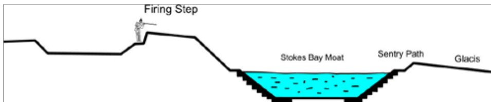
3.11 A section across the Stokes Bay Lines (Friends of Stokes Bay).
