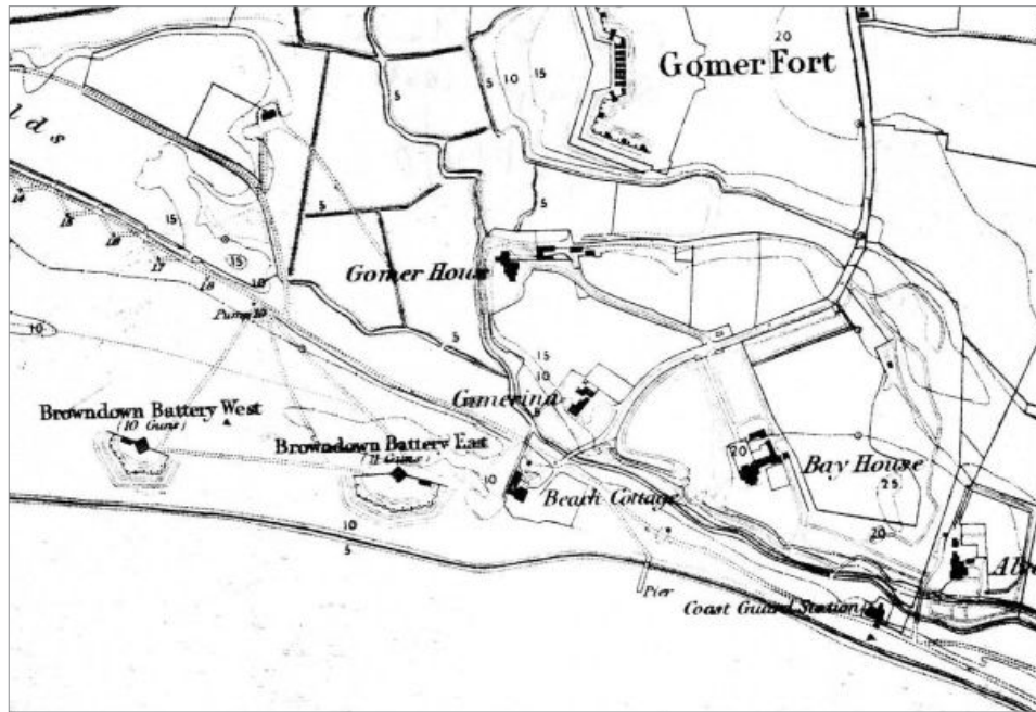
3.9 The Browdown batteries of 1852, surveyed in 1856 (fortgilkicker.co.uk).
