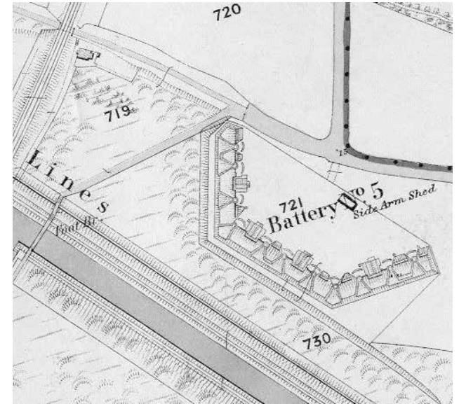
3.15 No. 5 Battery, as built, with the Lines shown on the seaward side (fortgilkicker.co.uk)
